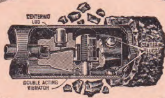
THE 'TORPEDO' FIRE TUBE CLEANER
