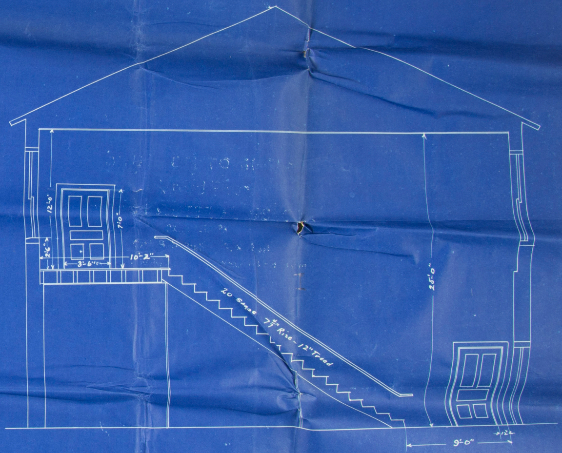
Section at Hall-way.
